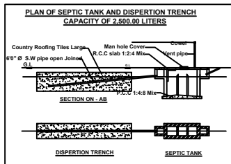
PLAN OF SEPTIC TANK AND DISPERSION TRENCH
