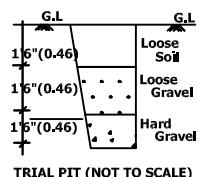
TRIAL PIT (NOT TO SCALE)
