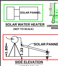
SIDE ELEVATION (NOT TO SCALE)
