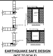
EARTHQUAKE SAFE DESIGN (NOT TO SCALE)
