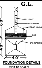
FOUNDATION DETAILS (NOT TO SCALE)
