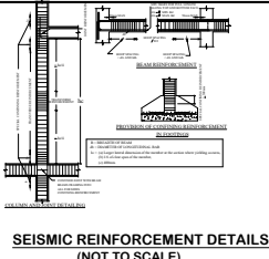
SEISMIC REINFORCEMENT DETAILS (NOT TO SCALE)
