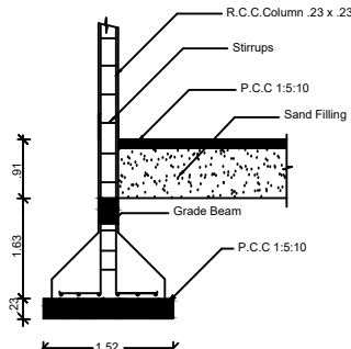
COLUMN DETAIL
