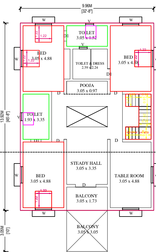
PRO.FIRST FLOOR PLAN
