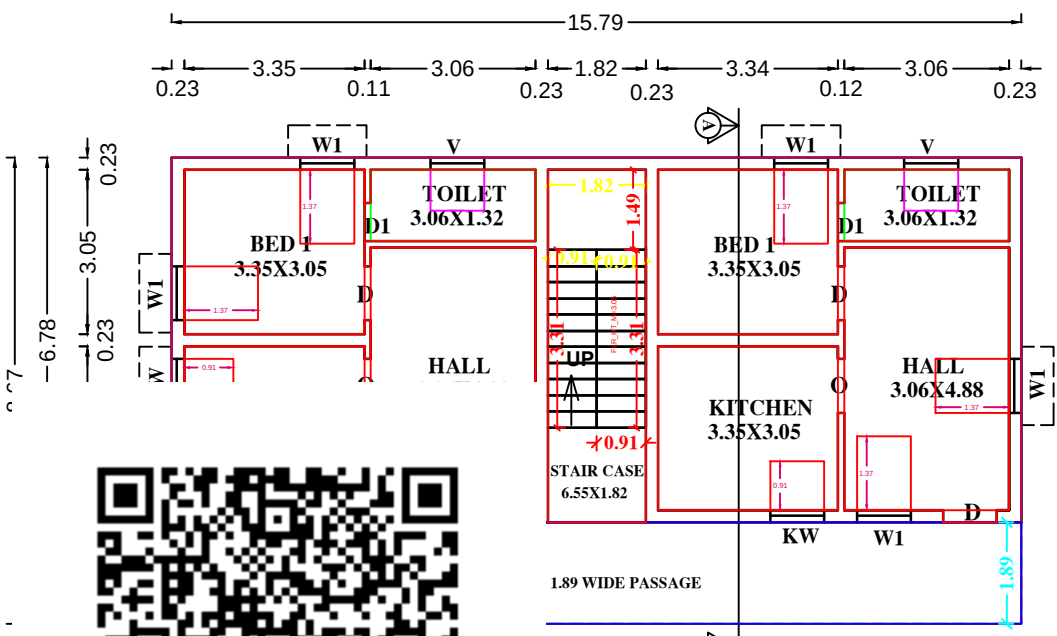
ND FLOOR PLAN
