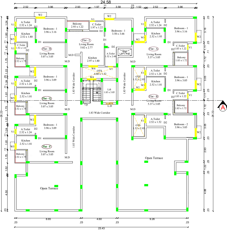
FIFTH FLOOR PLAN
