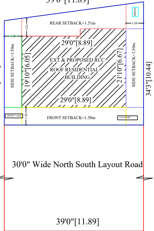
SITE PLAN
