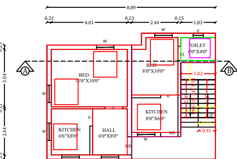
ALTERATION OF EXISTING FIRST FLOOR PLAN
