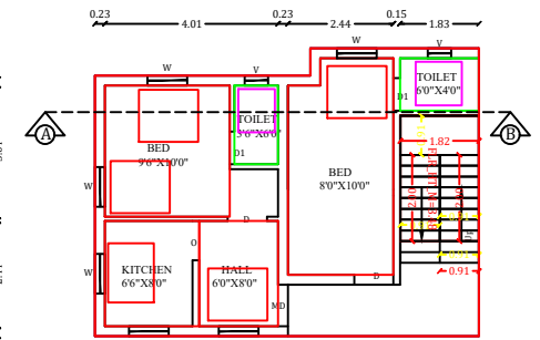
ALTERATION OF EXISTING FIRST FLOOR PLAN
