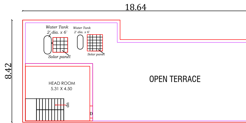
OPEN TERRACE PLAN
