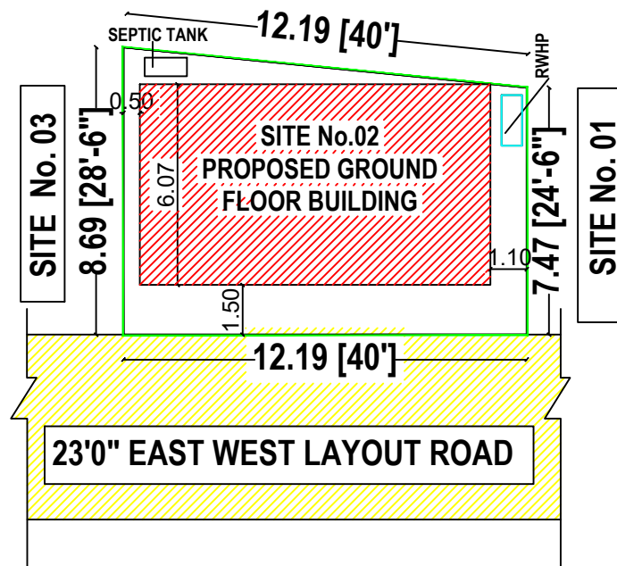
SITE PLAN
