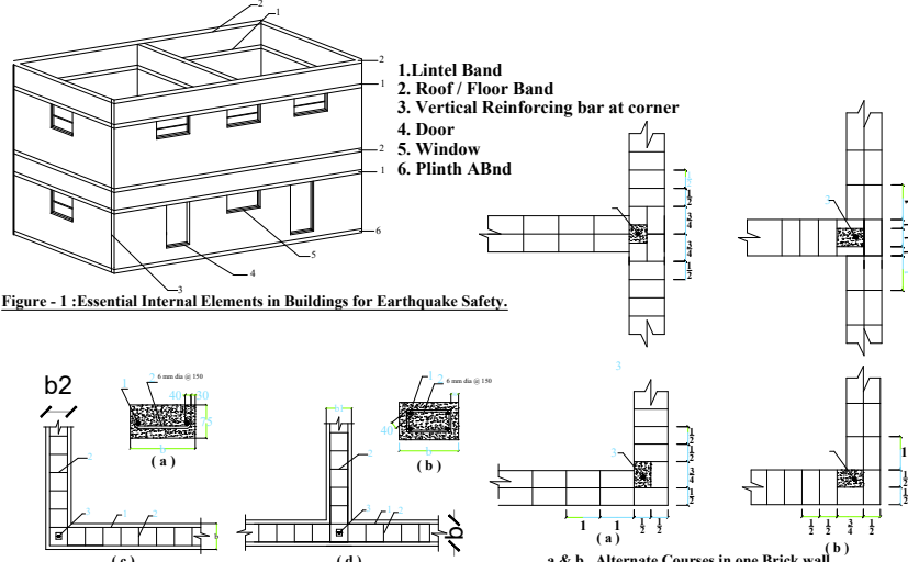
Figure - 3 : Typical Details of Providing Vertical Steel bars in Brick Masonry.
