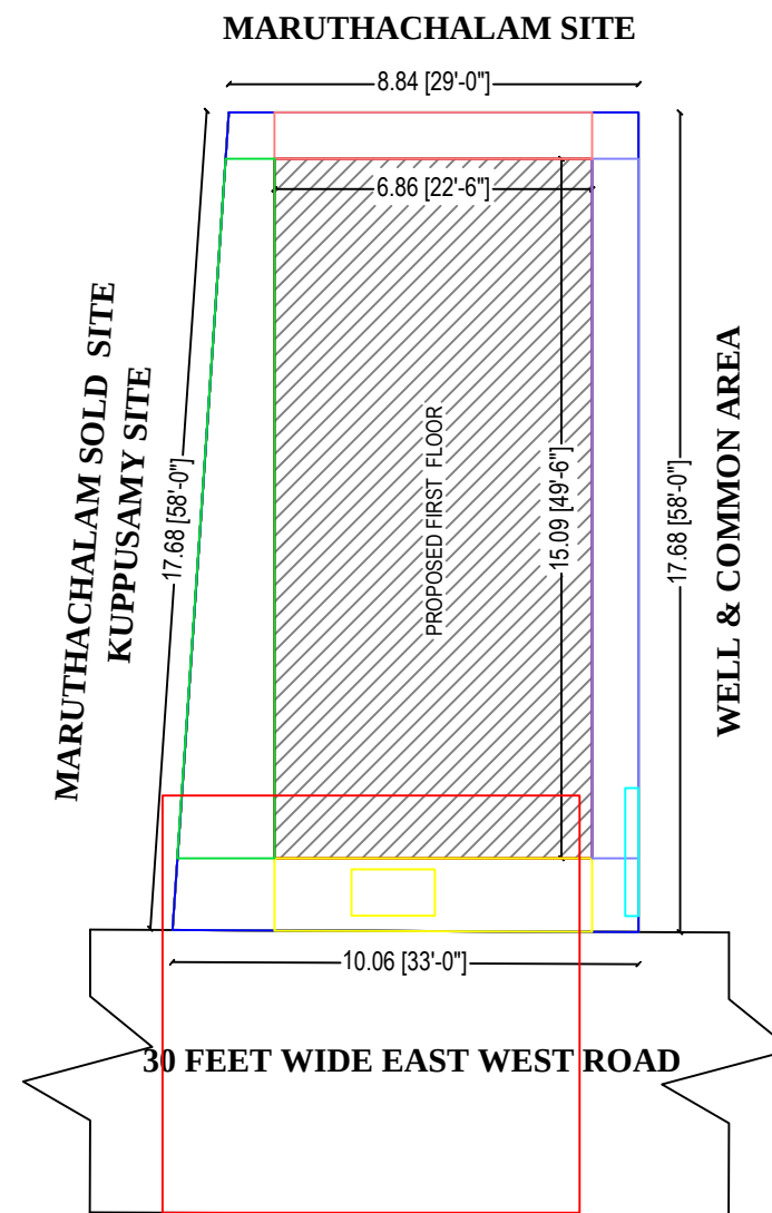
SITE PLAN
