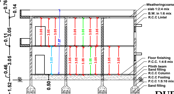
SECTION
