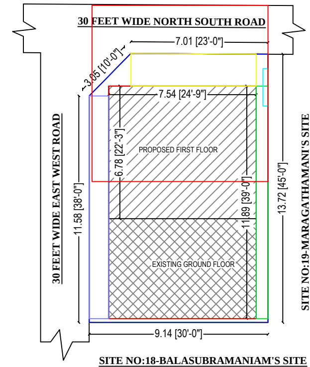
SITE PLAN
