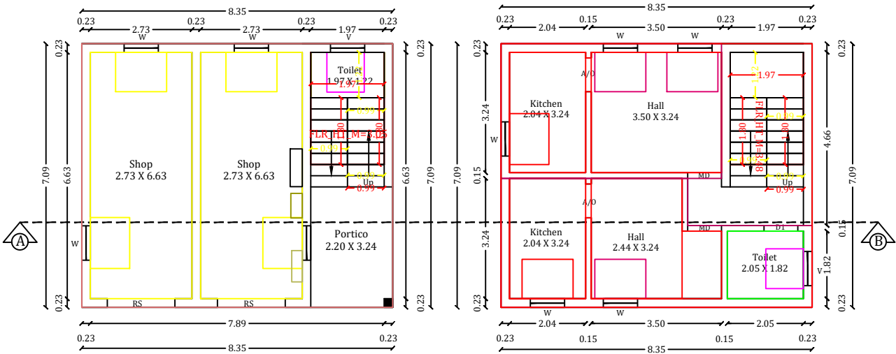
ALTERATION OF PROPOSED FIRST FLOOR PLAN
