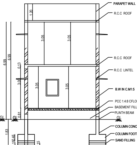
SECTION AB
