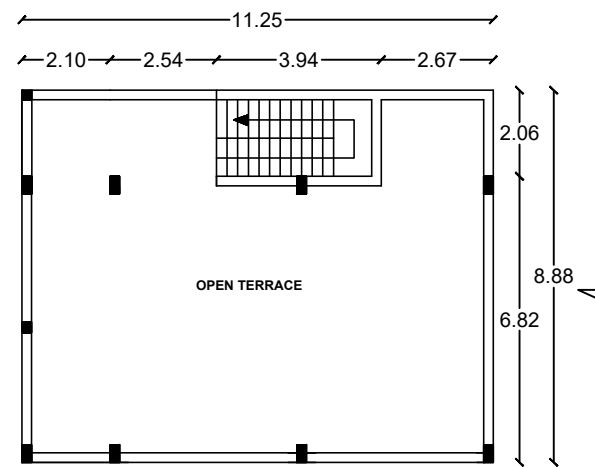
PRO. TERRACE FLOOR PLAN
