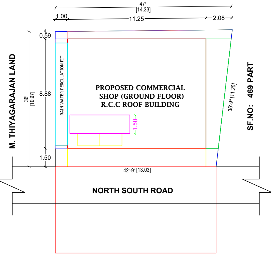
SITE PLAN
