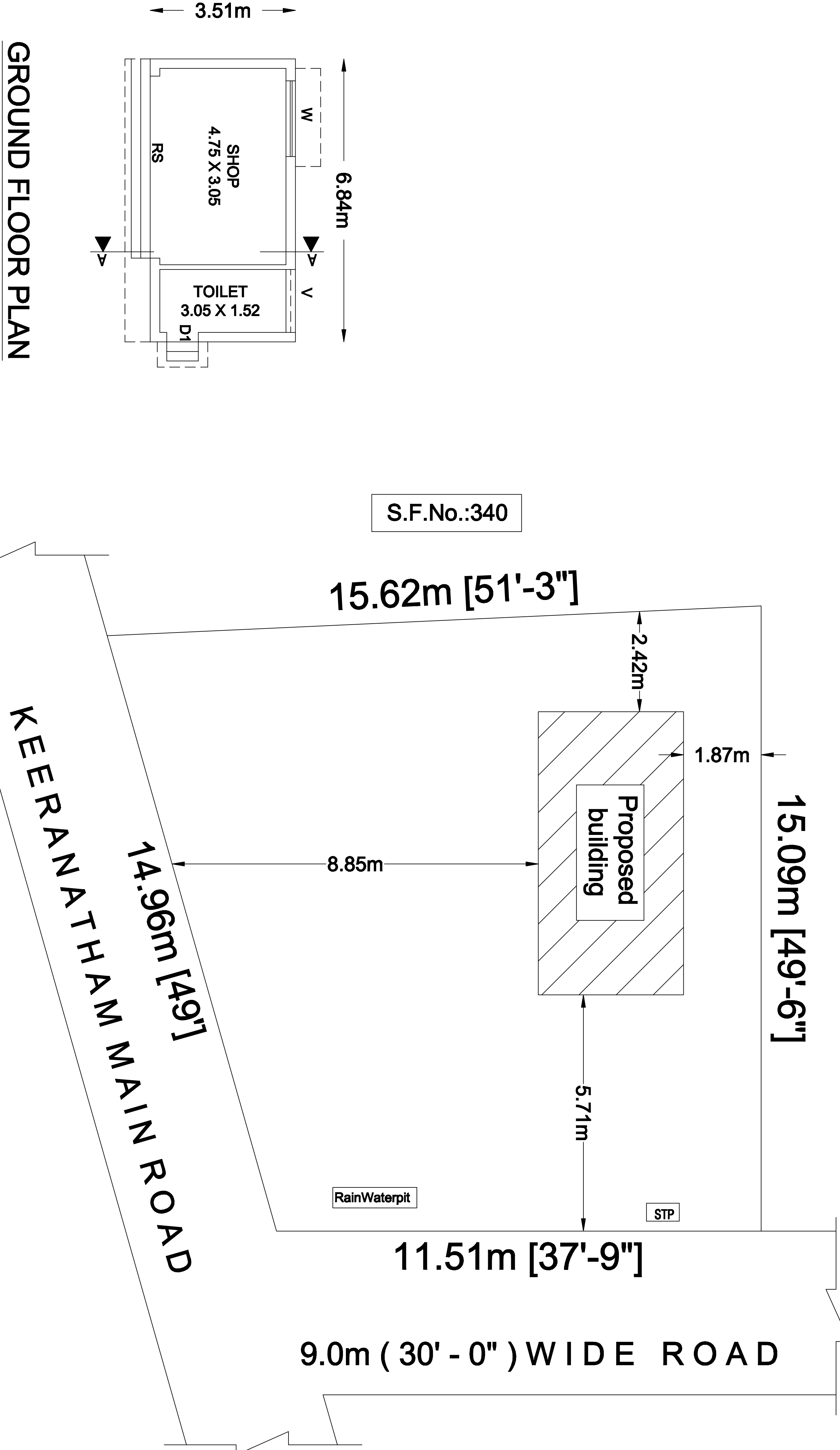
SITE PLAN
