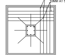
FOOTING DETAIL
