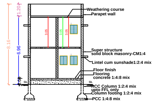
SECTION ELEVATION
