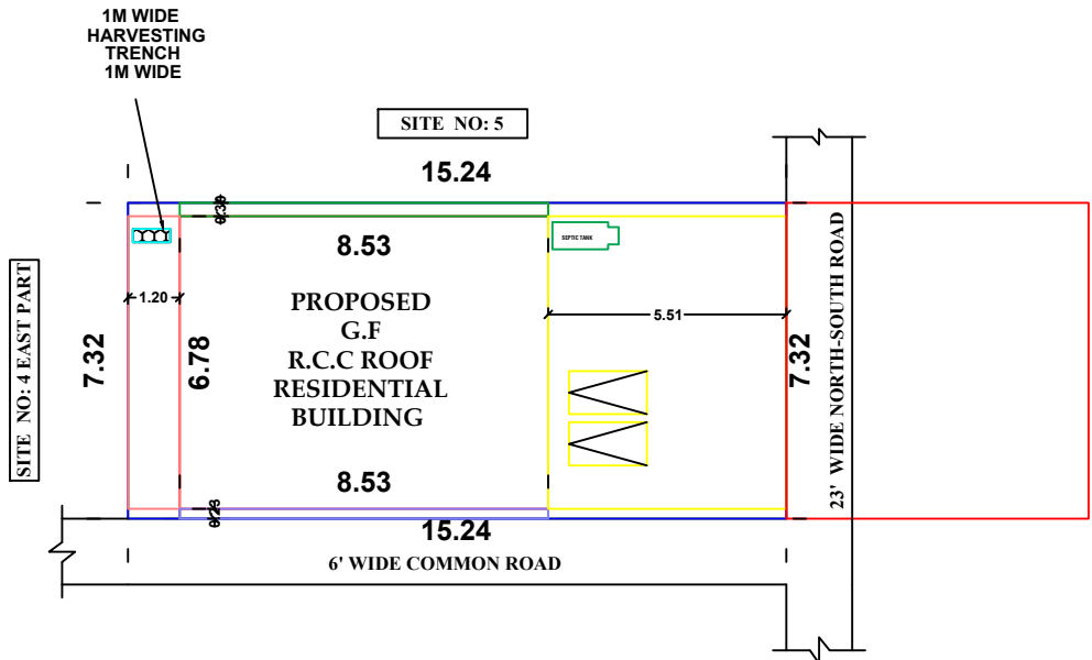
SITE PLAN
