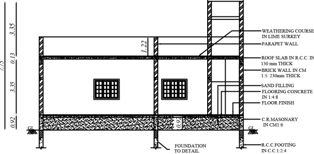
Eastern Side Section On "AB"
