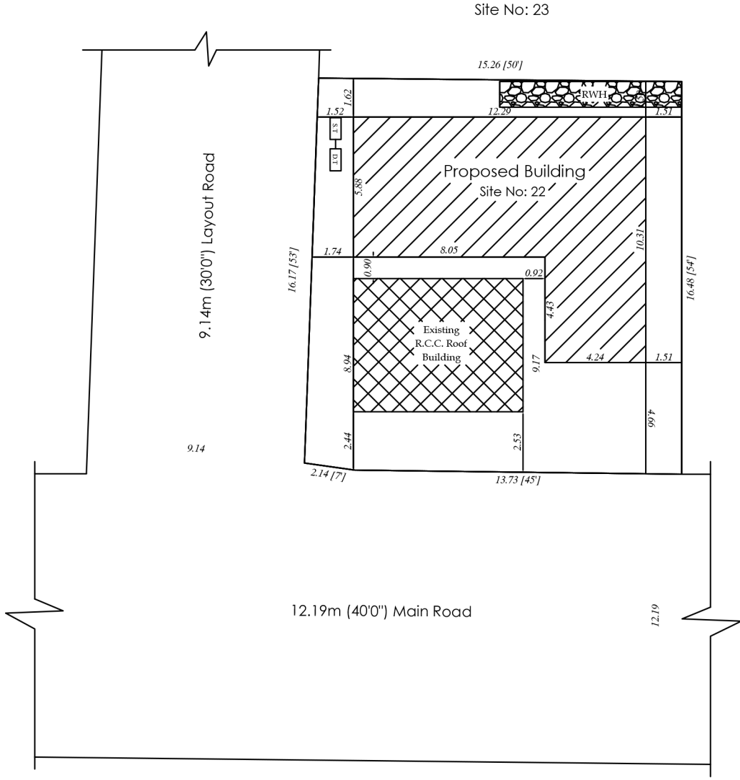
Site Plan
