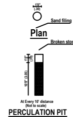
PERCOLATION PIT
