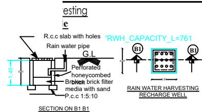
SECTION ON B1-B1
