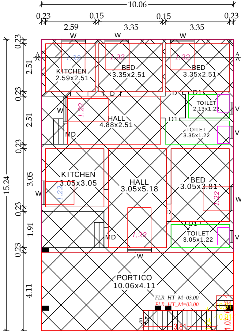
EXI. GROUND FLOOR PLAN
