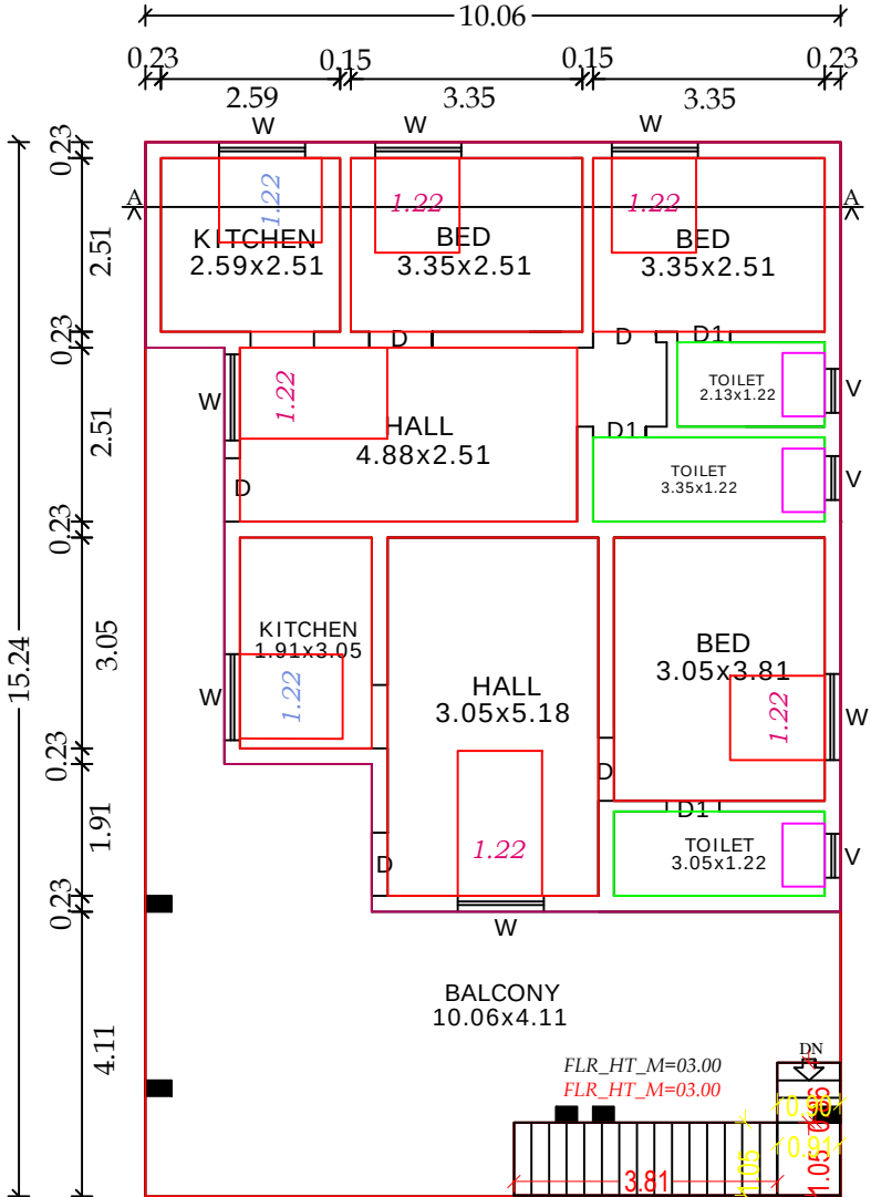
PRO. ADD. FIRST FLOOR PLAN
