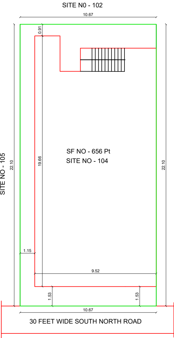
SITE PLAN
