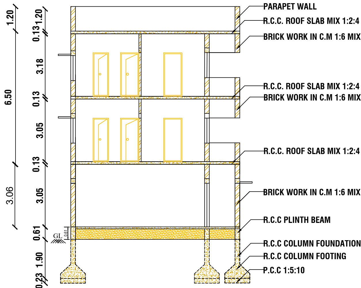
CROSS SECTION AT A-A
