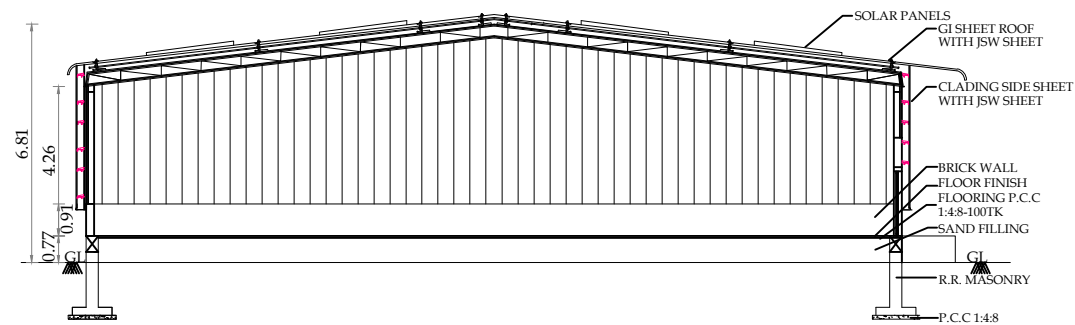
SECTION 'AA' BLOCK - 1
