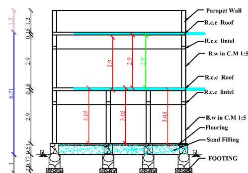
SECTION AB
