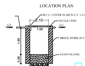
RAIN WATER COLLECTION PIT
