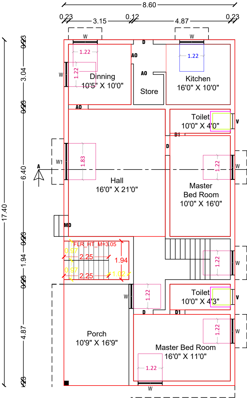
GND FLOOR PLAN
