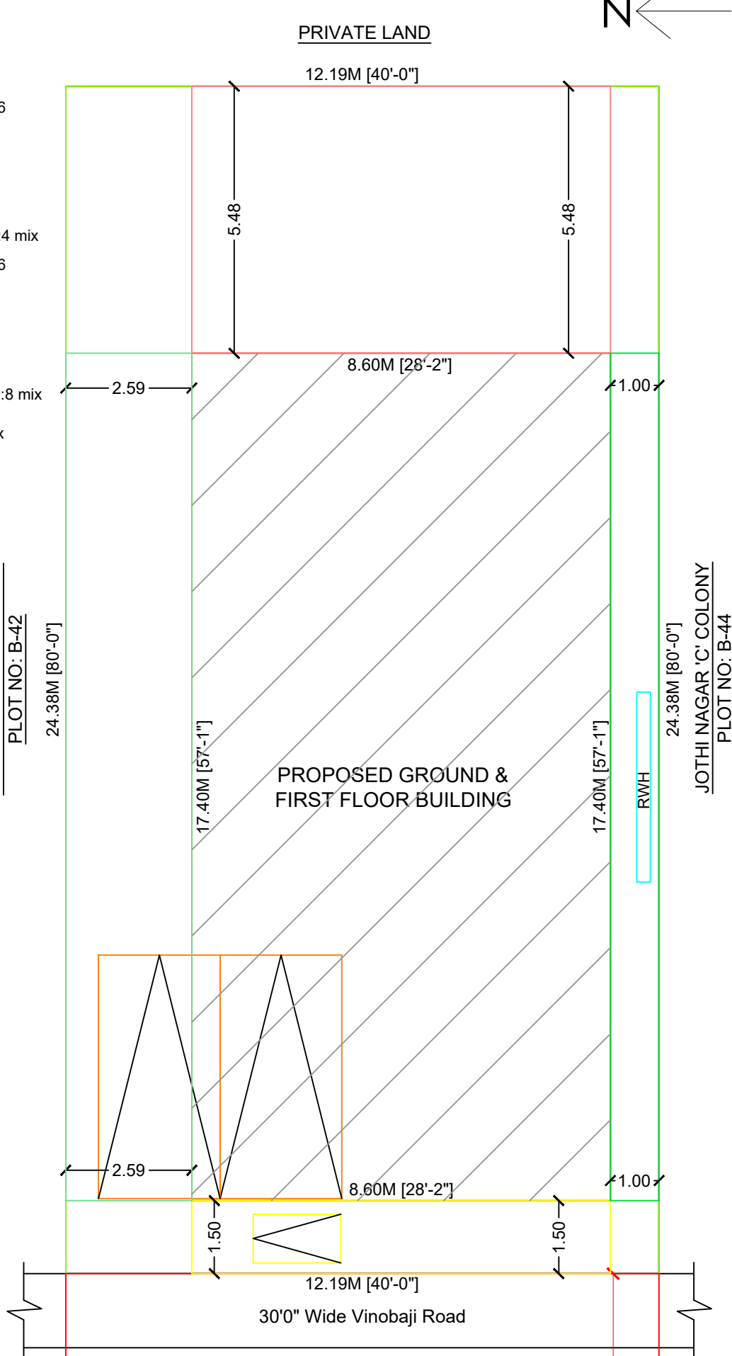
SITE PLAN
