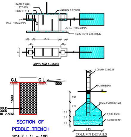
COLUMN DETAILS
