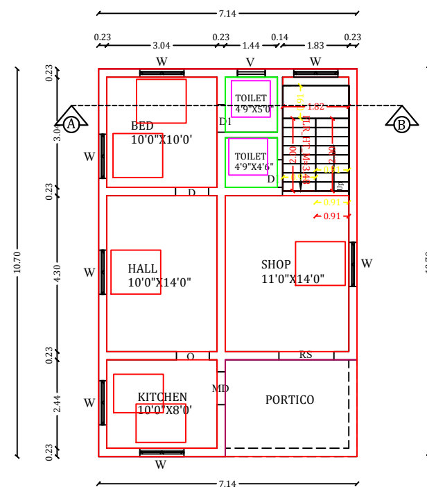
ADDITION & ALTERATION OF GROUND FLOOR PLAN
