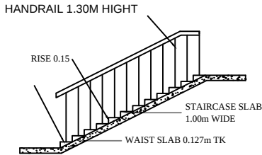
STAIRCASE DETAILS
