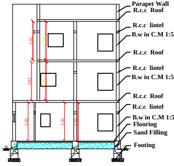
SECTION AB
