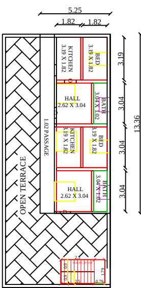
ADD. PROPOSED SECOND FLOOR PLAN
