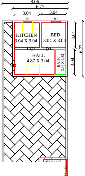
LOOR PLAN
