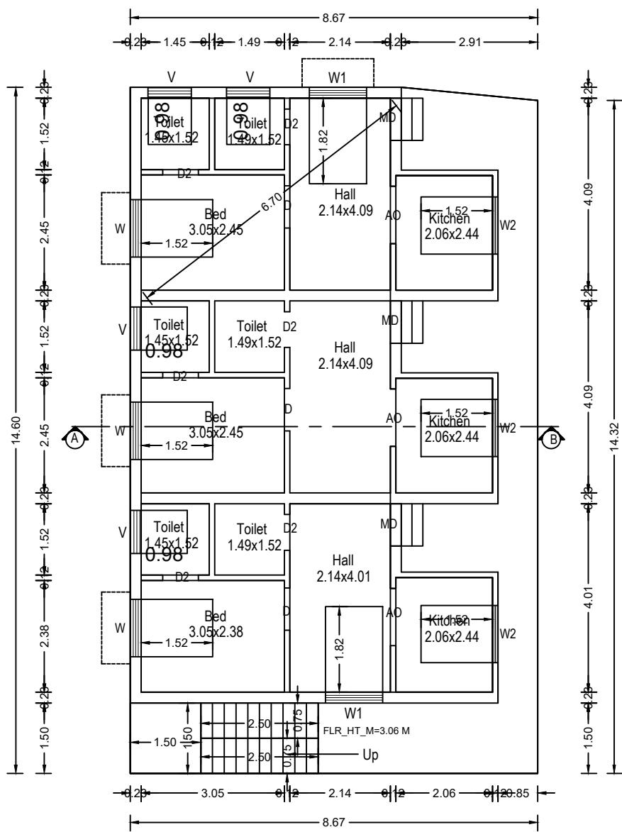
Plan Scale 1:100
