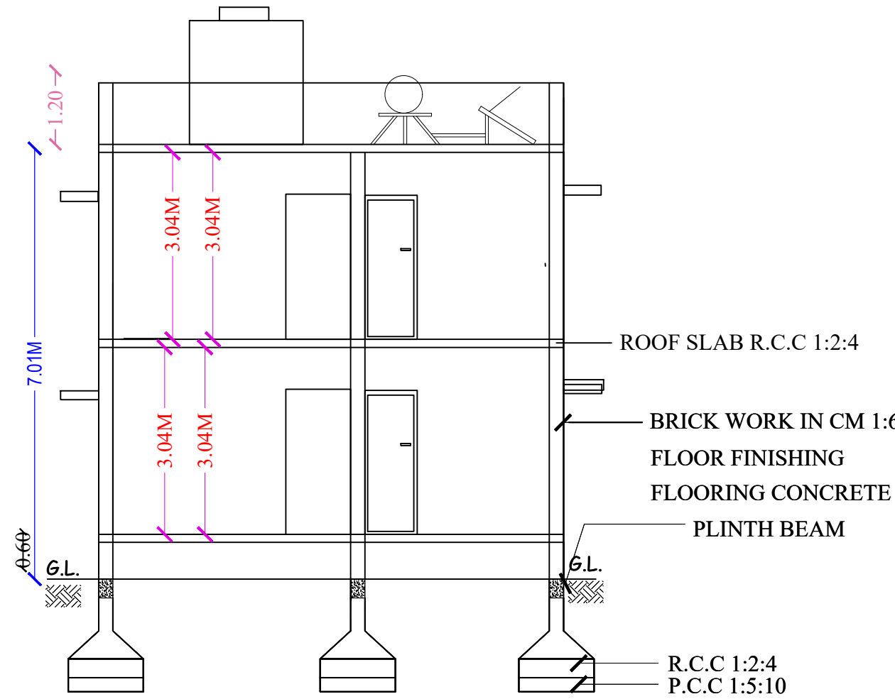
SECTION "A-A"
