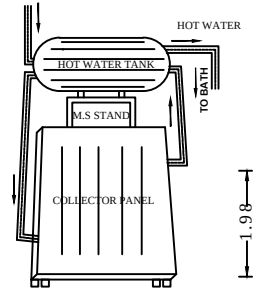
SOLAR WATER HEATER SYSTEM
