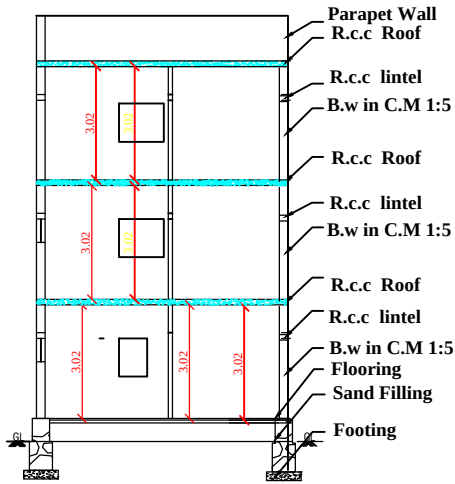
SECTION AB
