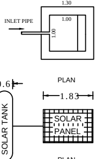
SOLAR SYSTEM
