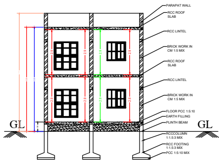
SECTION AB
