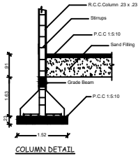
COLUMN DETAIL
