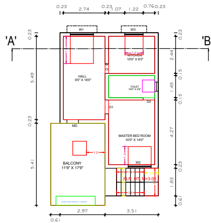
PROPOSED FIRST FLOOR
