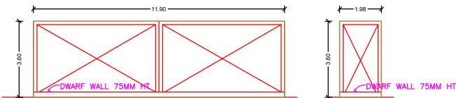
MAIN GATE
