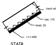
STAIR
