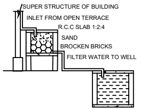
RAINWATER HARVESTING
