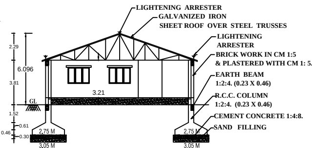
SCETION ON 'A-B'
