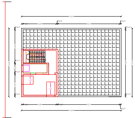
PRO. FIRST FLOOR PLAN
