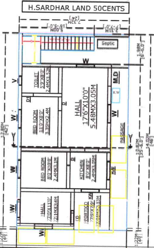
Site Cum Ground Floor Plan
