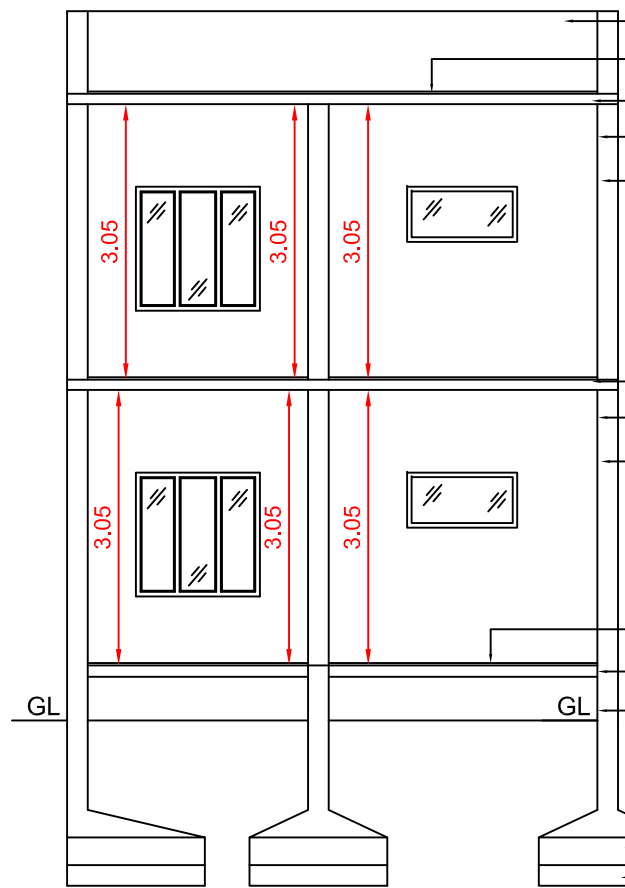
CROSS SECTION ON XY
