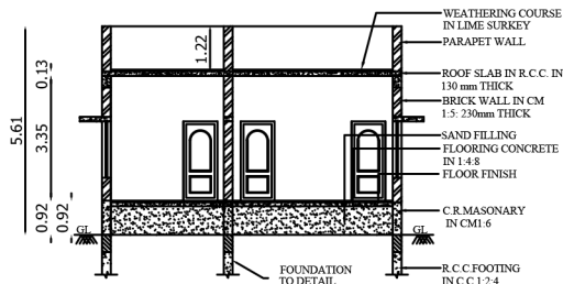
Easte Side Section On "AB"
