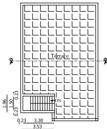
Head Room Plan
