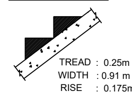
STAIRCASE DETAIL:
