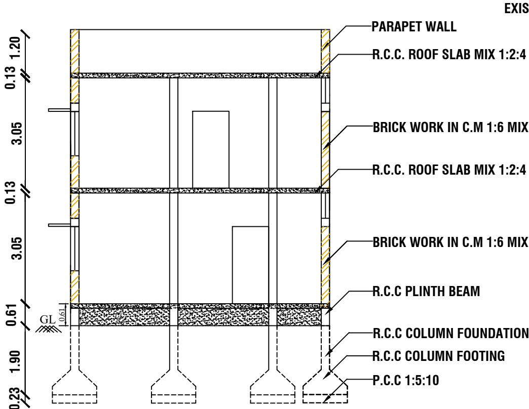
CROSS SECTION AT A-A
