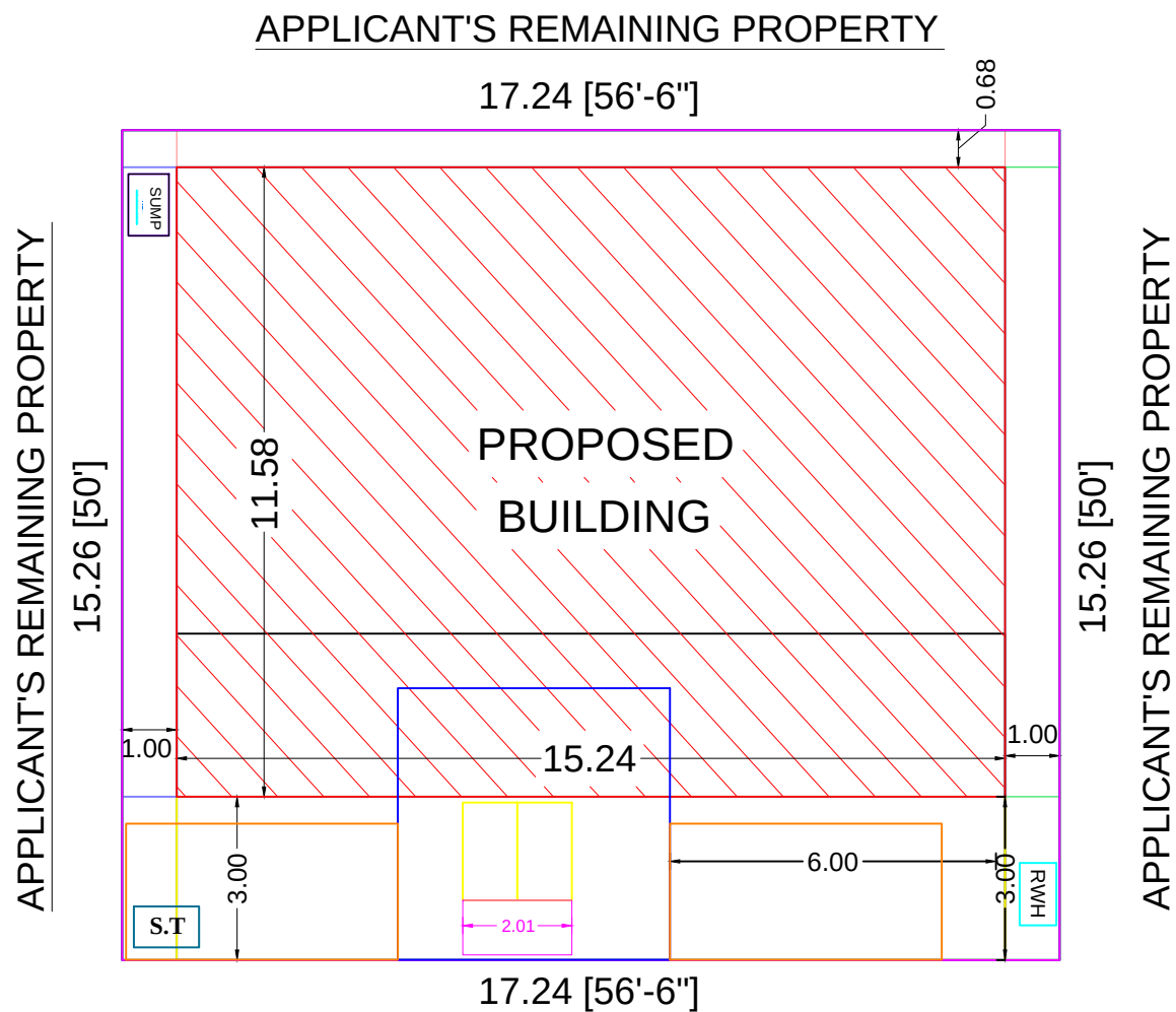
CONCERN SITE PLAN
