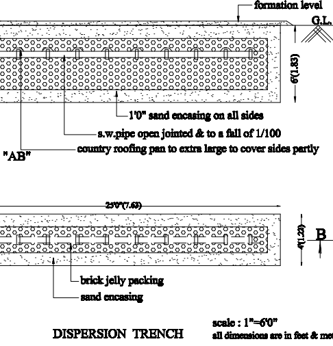
PLAN SHOWING THE DETAILS OF SEPTIC TANK 450 GALLONS (2043 LIT.) CAPACITY WITH DISPERSION TRENCH
