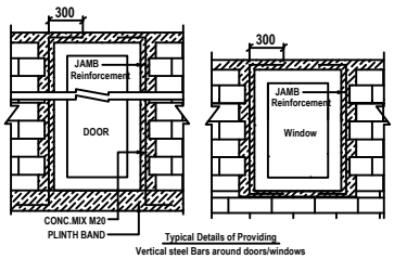
Typical Details of Providing Vertical steel Bars around doors/windows
