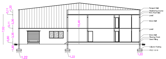
SECTION ON B B
