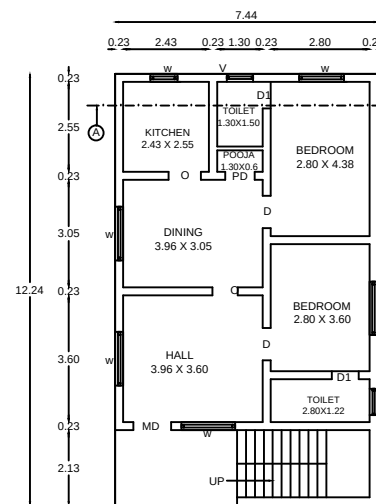
ADD. PROPOSED FIRST FLOOR
