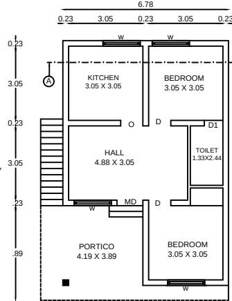
EXISTING GROUND FLOOR
