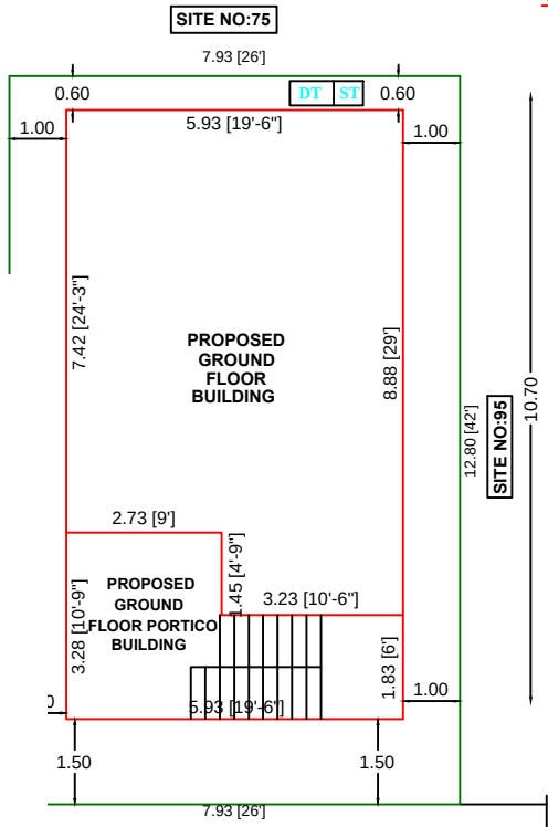
SITE PLAN
