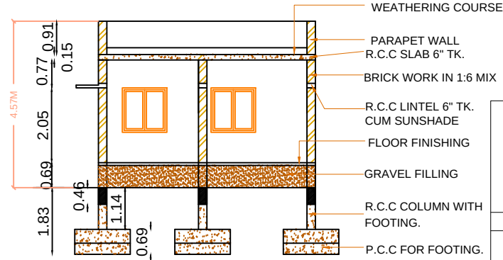
CROSS SECTION AT A-A
