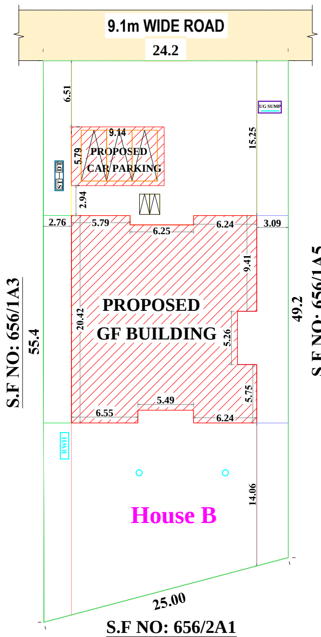
SITE PLAN
